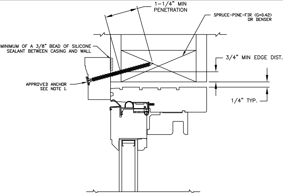
TYPICAL BRICKMOULD/FLAT CASING WINDOW HEAD JAMB
